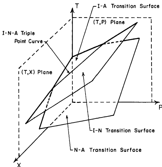
Figure 1. Illustration of three phase transition surfaces and a curve of triple points. The I, N, and S_A phases exist in the regions above, between, and below the surfaces, respectively. The phase diagram for a pressure experiment and mixing experiment are shown by the bold lines on the ( T, P ) plane and ( T, X ) plane, respectively.
