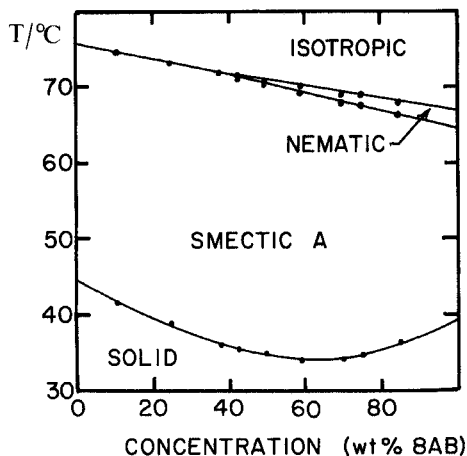
Figure 3. Temperature-concentration phase diagram for the 9AB/8AB system. A triple point occurs at 71.5 \pm 0.5^\circ\text{C} and 38 \pm 2 \text{ wt}\% \text{ 8AB} .
